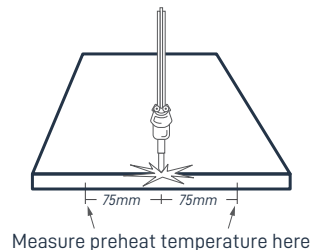
Figure 1: Recommended preheat zone and location of preheat measurement.
